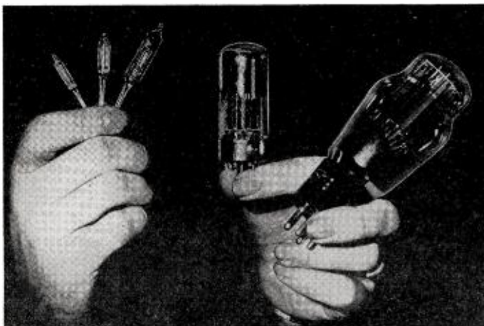
TINY TUBE (extreme l), constructed in Advance Development Laboratories of Sylvania Electric Products Inc., is described by its manufacturers as "smallest radio tube in the world." Only \frac{1}{8} of an inch long and slightly more than \frac{1}{16} inch in diameter, it is shown in comparison with (r to l) the conventional tube of ten years ago, current lock-in tube and the proximity fuze tube. Sylvania produced more than 140 million proximity fuze tubes during the war.
